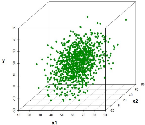
3D Scatterplot
